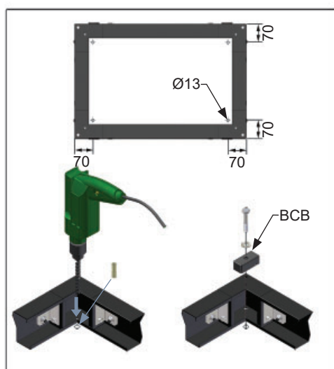
Clamping Bracket (Internal fixing)
